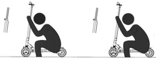
If the main rod of the electric scooter shakes during running, please use a M10 hexagon wrench to tighten the bolts at the fold mechanism.
